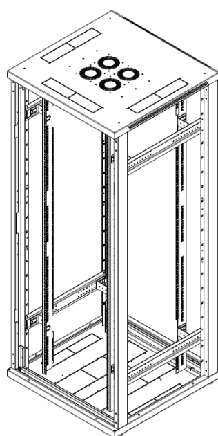
3D REAR VIEW OPEN FRAME
