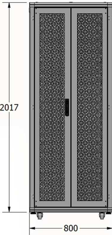
Front View
